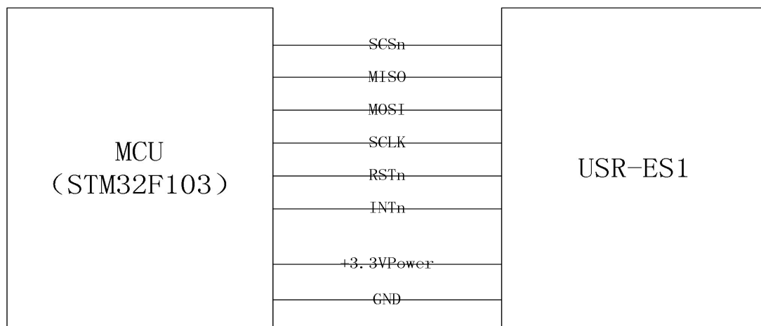
Diagram 5-1 Connection Diagram
